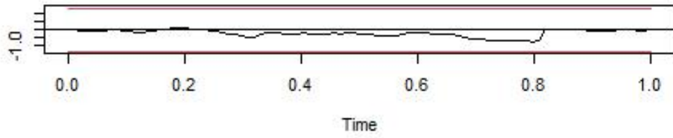
OLS-CUSUM of equation PC1
