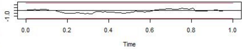
OLS-CUSUM of equation PC4
