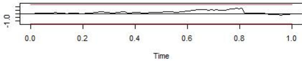
OLS-CUSUM of equation PC3
