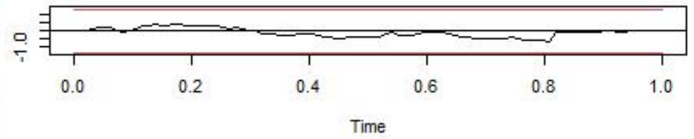
OLS-CUSUM of equation PC5
