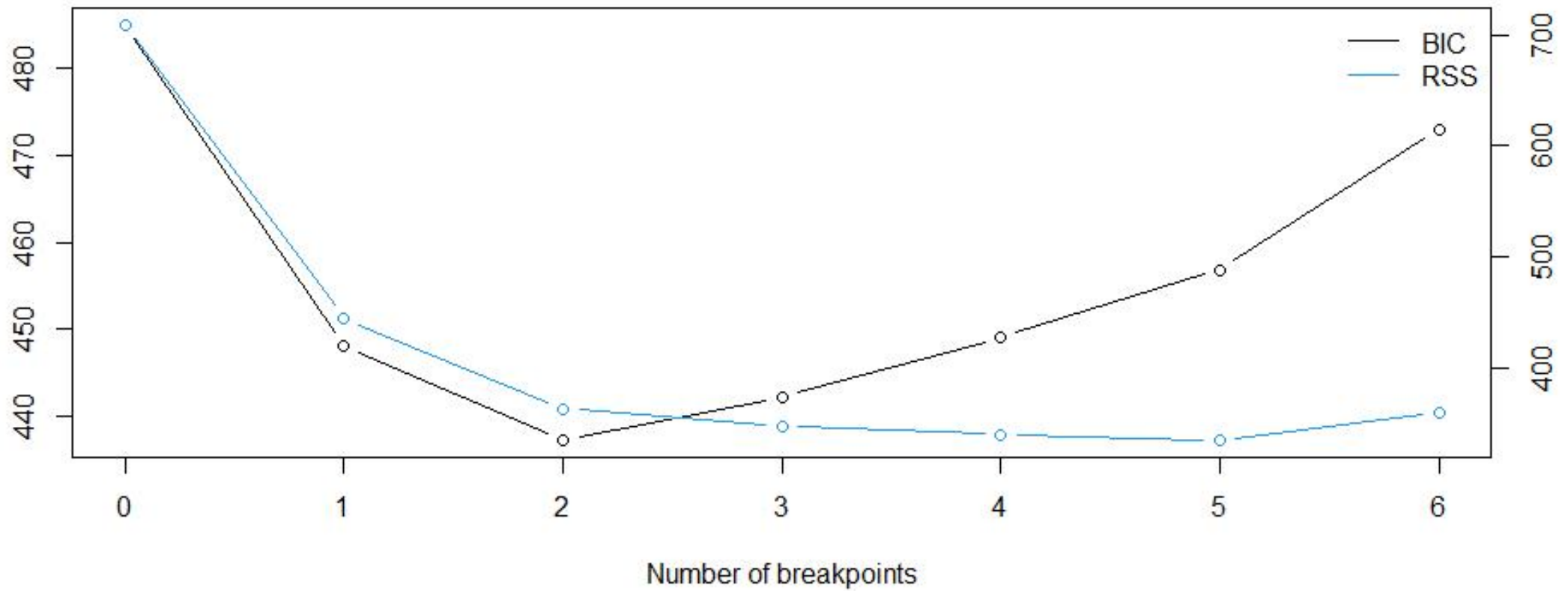
BIC and Residual Sum of Squares
