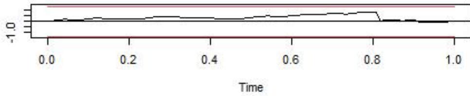
OLS-CUSUM of equation PC2
